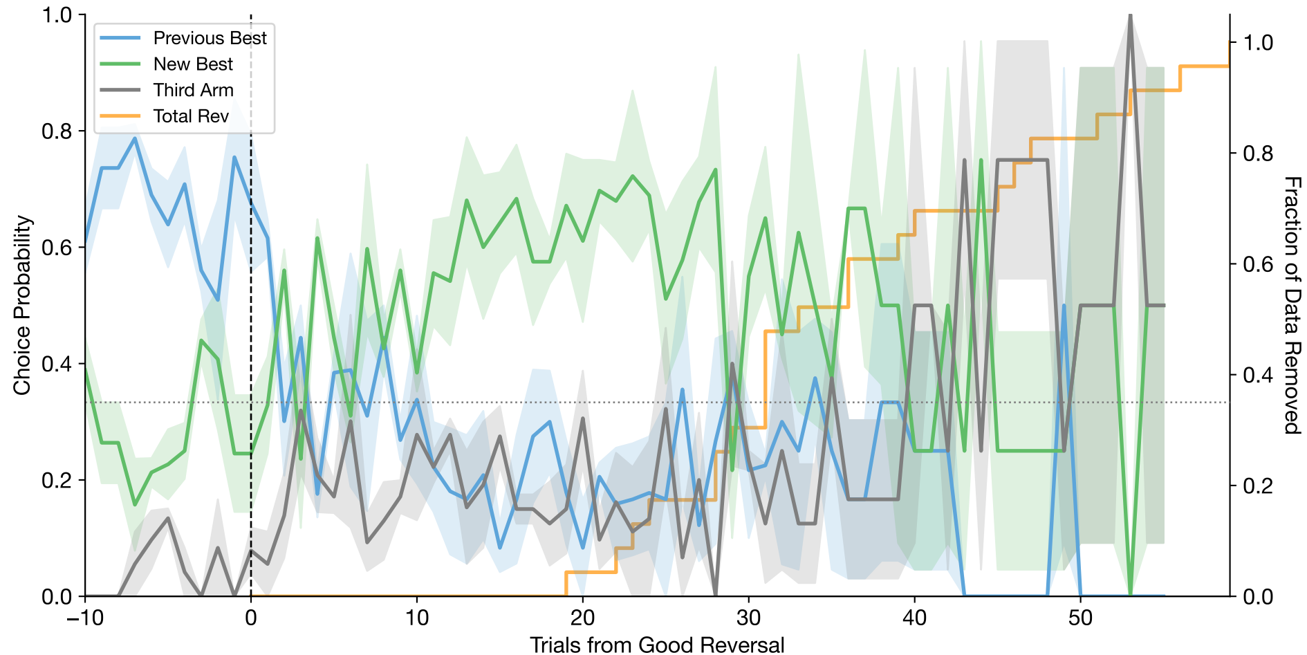
Good Reversal-Aligned Choices (mean \pm se across subjects | n=3 subjects, n=23 reversals)
